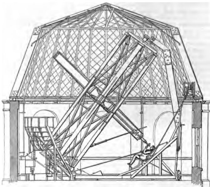
THE NORTHUMBERLAND TELESCOPE.
